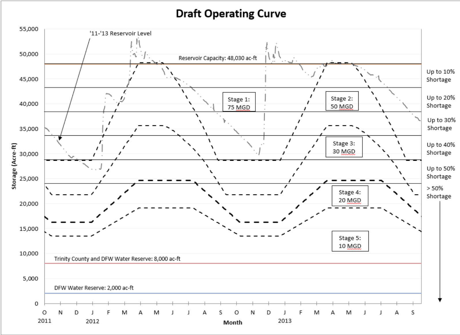
Figure 8: Ruth Lake operating curves with 2011-2013 Reservoir Levels
