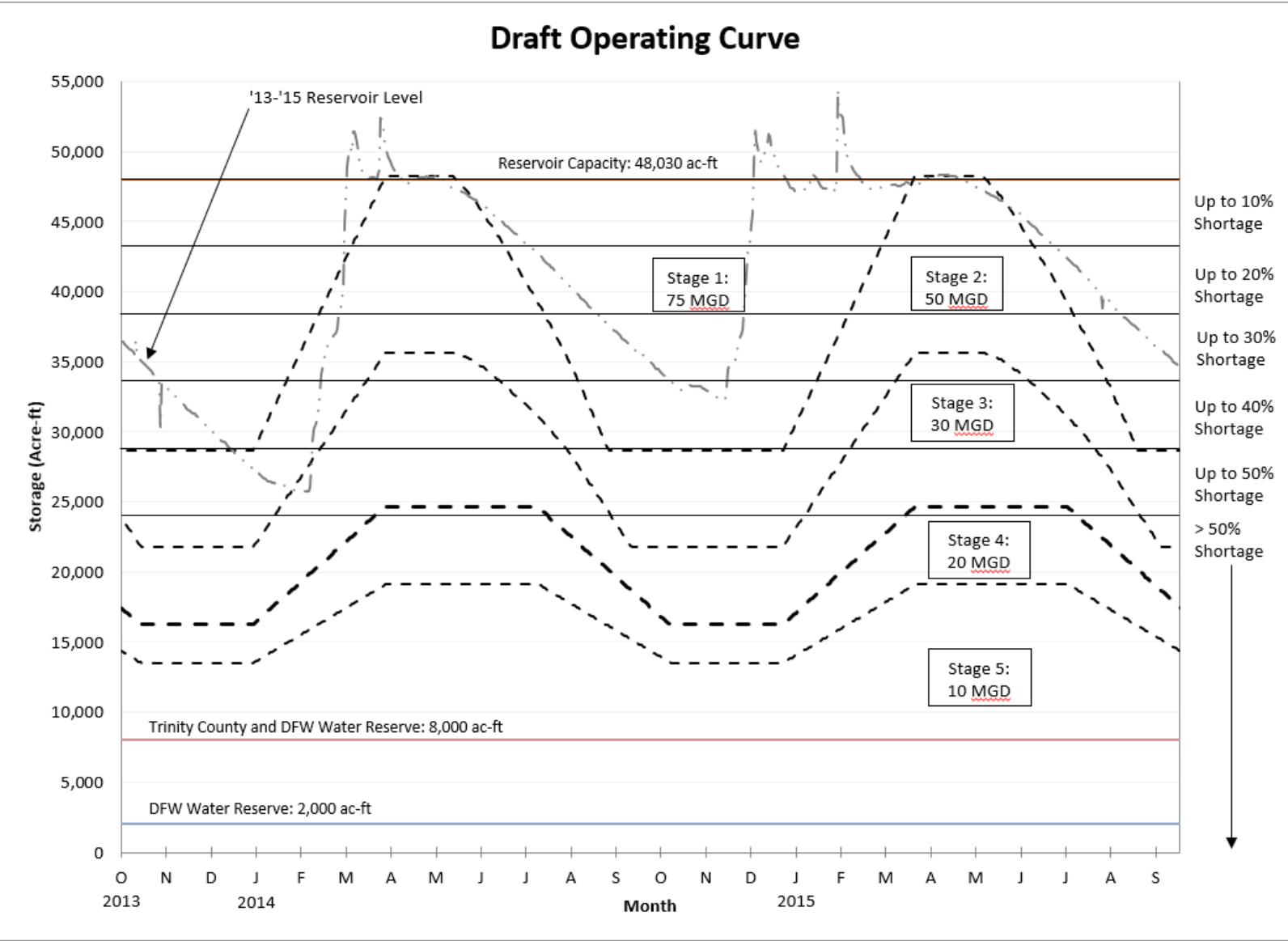
Figure 9: Ruth Lake operating curves with 2013-2015 Reservoir Levels
